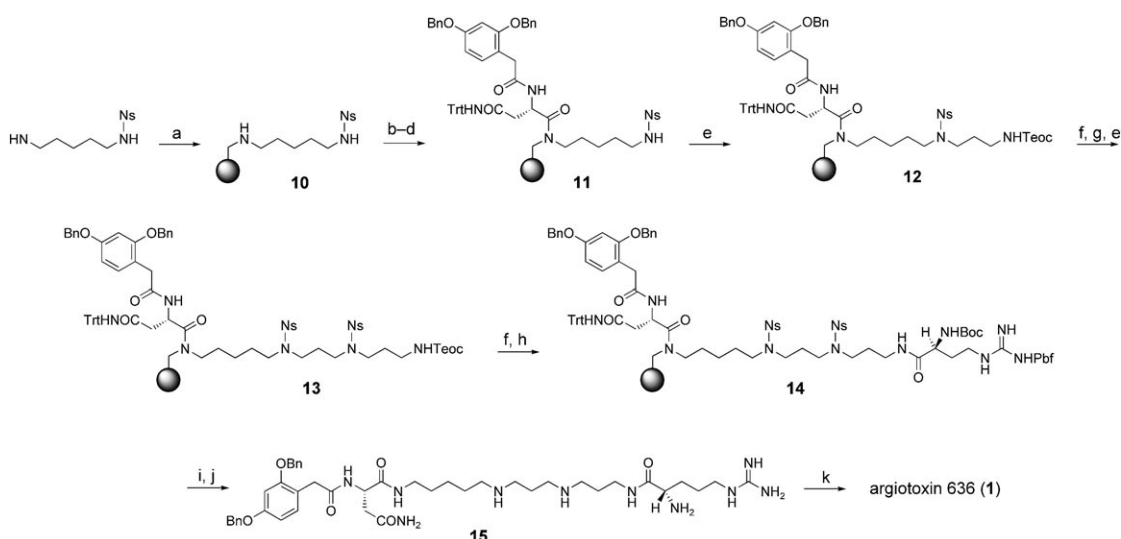
Scheme 2. Solid-phase synthesis of ArgTX-636 ( 1 ): a) BAL PS resin (loading: 0.92 \text{ mmol g}^{-1} ), \text{NaCNBH}_3 , DMF/AcOH (99:1), 1 h; b) Fmoc-L-Asn(Trt)-OH, HATU, collidine, DMF, 16 h followed by purification/washing and a further 16 h; c) 20% piperidine in DMF, 2 min followed by purification/washing and a further 20 min; d) 2-(2,4-bis(benzyloxy)phenyl)acetic acid, HATU, collidine, DMF, 2 h; e) \text{HO}(\text{CH}_2)_3\text{NHTeoc} , \text{Bu}_3\text{P} , ADDP, \text{CH}_2\text{Cl}_2/\text{THF} (1:1), 3 \times 3 \text{ h} ; f) TBAF, THF, 50^\circ\text{C} , 30 min; g) Ns-Cl, THF/ \text{CH}_2\text{Cl}_2 (2:1), 3 h; h) Boc-L-Arg(Pbf)-OH, HATU, collidine, DMF, 2 h; i) DBU, \beta -mercaptoethanol, DMF, 3 \times 20 \text{ min} ; j) TFA/ \text{CH}_2\text{Cl}_2/\text{TIS}/\text{H}_2\text{O} (47.5:47.5:2.5:2.5), 2 h; k) \text{H}_2 , Pd/C, MeOH, 16 h. ADDP = 1,1'-azodicarbonyldipiperidine, Bn = benzyl, Boc = tert -butoxycarbonyl, DBU = 1,8-diazabicyclo[5.4.0]undecane, DMF = N,N -dimethylformamide, Fmoc = 9-fluorenylmethoxycarbonyl, HATU = N -((dimethylamino)-1 H -1,2,3-triazolo[4,5- b ]pyridin-1-ylmethylene)- N -methylmethanaminium hexafluorophosphate N -oxide, Ns = o -nitrobenzenesulfonyl, Pbf = 2,2,4,6,7-pentamethyl-2,3-dihydro-1 H -benzofuran-5-sulfonyl, TBAF = tetrabutylammonium fluoride, Teoc = 2-trimethylsilylethoxycarbonyl, TIS = triisopropylsilane, TFA = trifluoroacetic acid, Trt = trityl.
